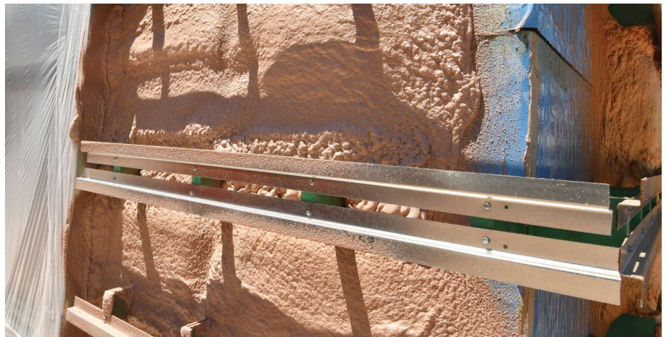
Insulthane Extreme featuring Solstice LBA was applied on the exterior walls to provide outstanding thermal performance and air tightness.
